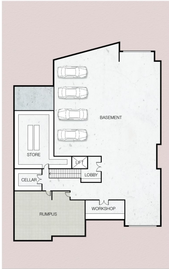
BASEMENT PLAN
